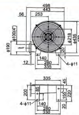
HTB75-105 6-stage
