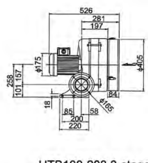
HTB100-203 3-stage
