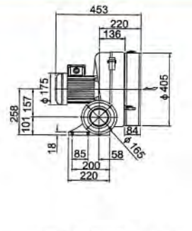
HTB100-102 2-stage
