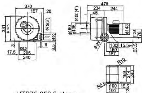
HTB75-053 3-stage
