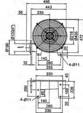
HTB100-304 4-stage
