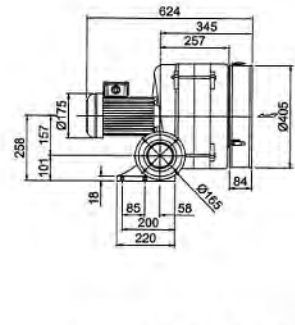
HTB100-304 4-stage
