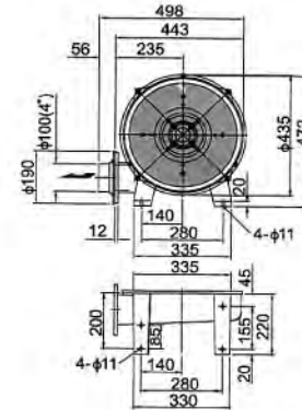
HTB100-505 5-stage
