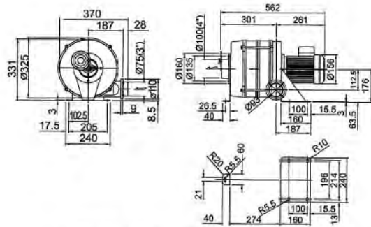
HTB75-104 4-stage
